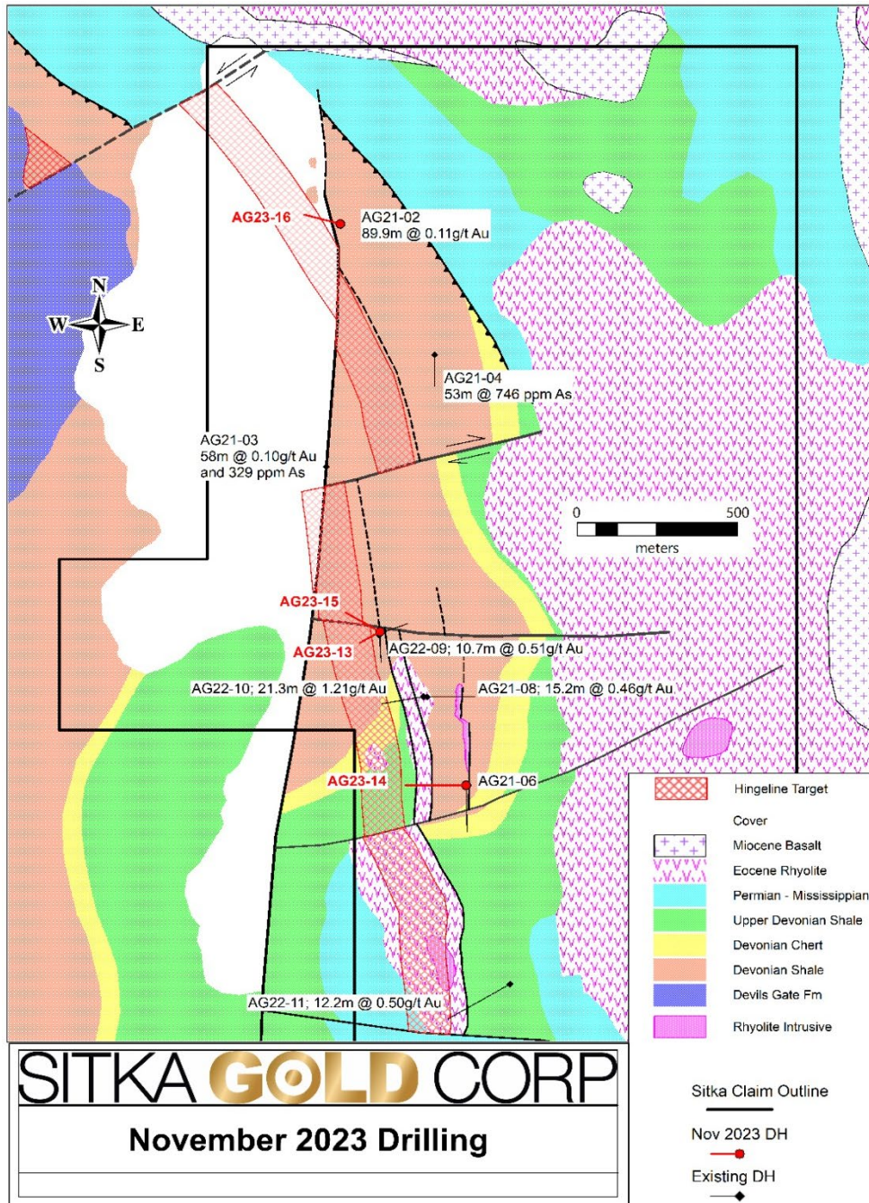
Figure 2: Alpha Claim Block, Geology, Alteration, Drill Collar Locations
