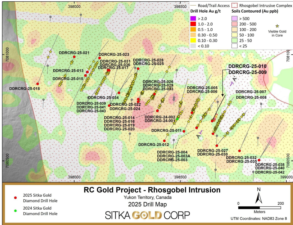
Figure 4: Plan map of the Rhosgobel intrusion showing the 2025 drilling.
