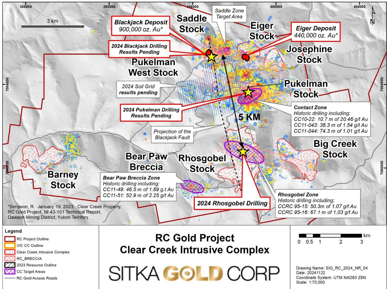
Fig 2 Clear Creek Intrusive Complex
