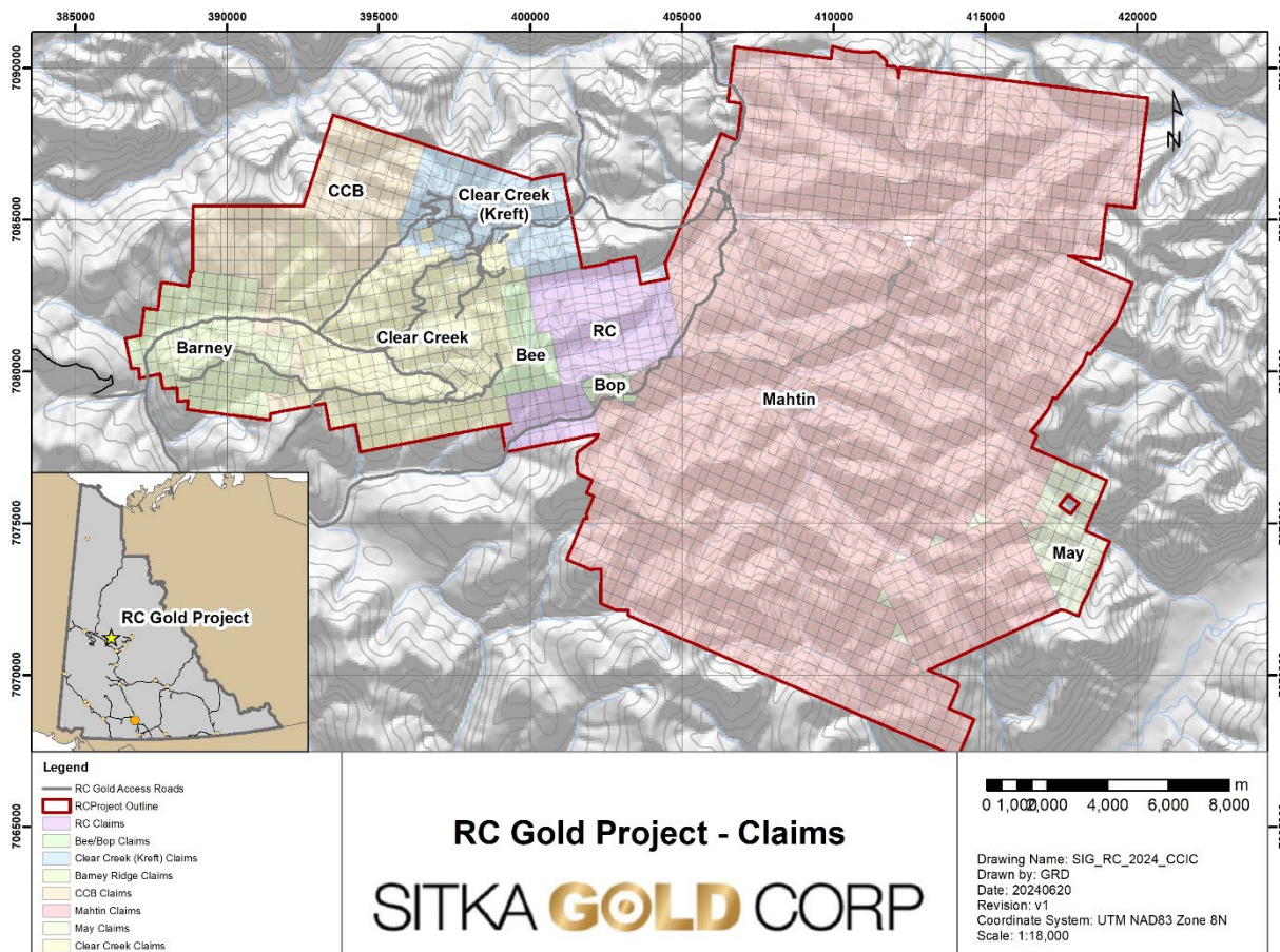
Figure 1 RC Gold Project Claim Map
