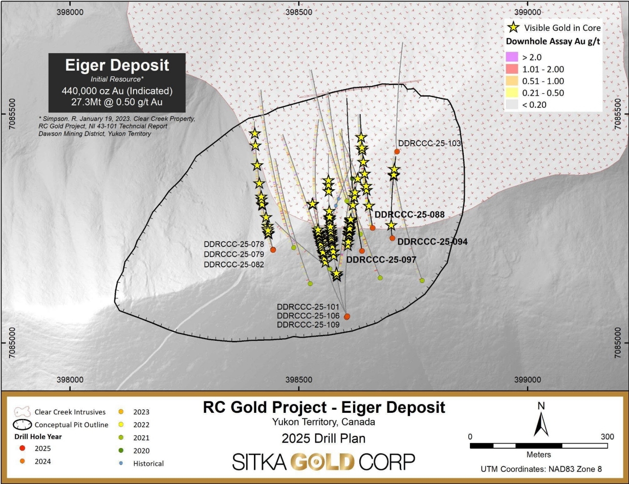
Figure 3: Plan map of drilling at the Eiger Zone. 10 drill holes have been completed at Eiger in 2025 with multiple occurrences of visible gold observed in the drill core (yellow stars).
