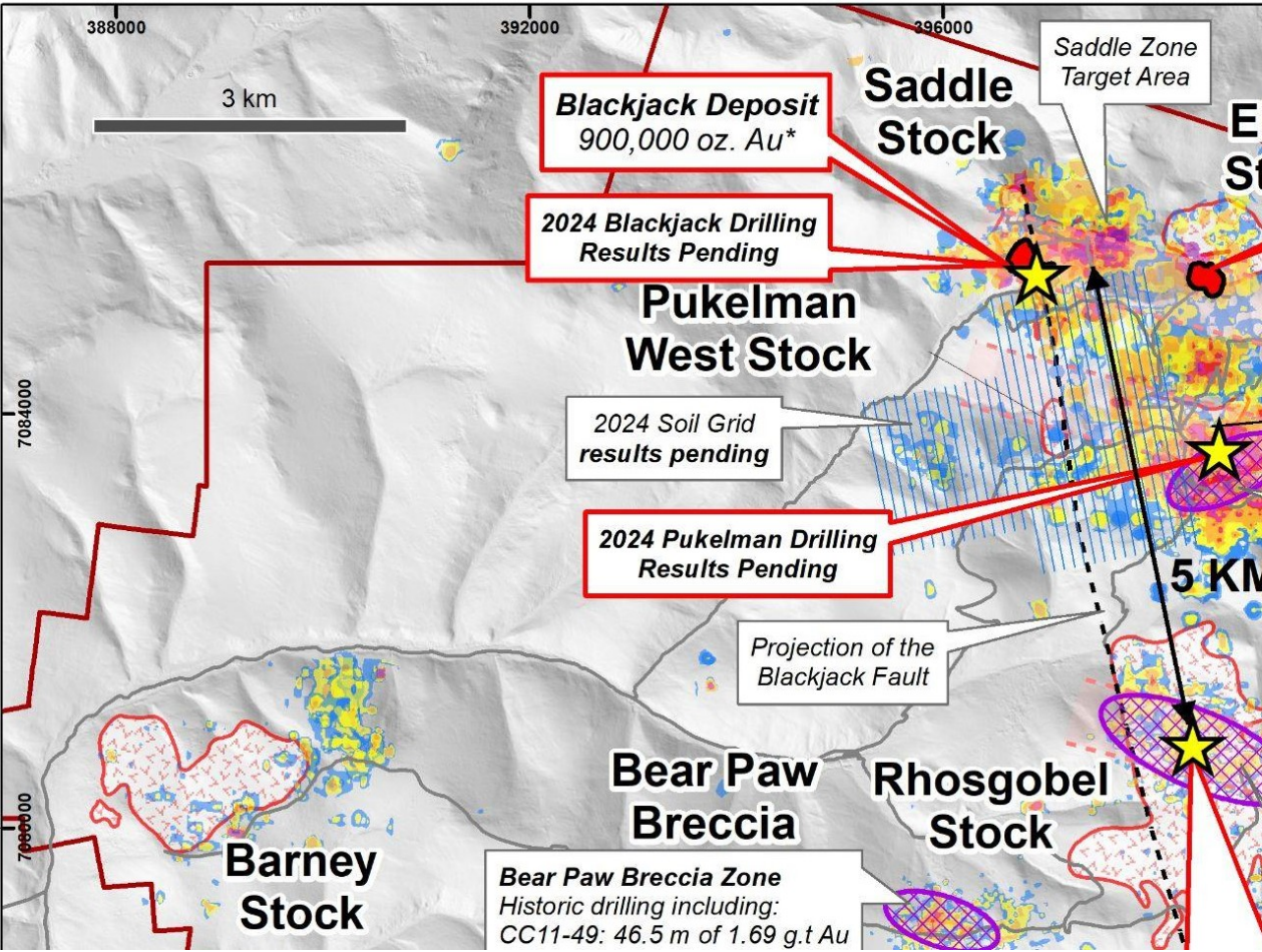
Fig 3 Clear Creek Intrusive Complex
