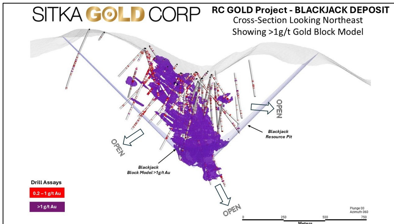
Figure 2B: Block Model of the Blackjack resource illustrating the coherent core of greater than 1 g/t material that extends from surface to a currently defined depth of 660 m.
