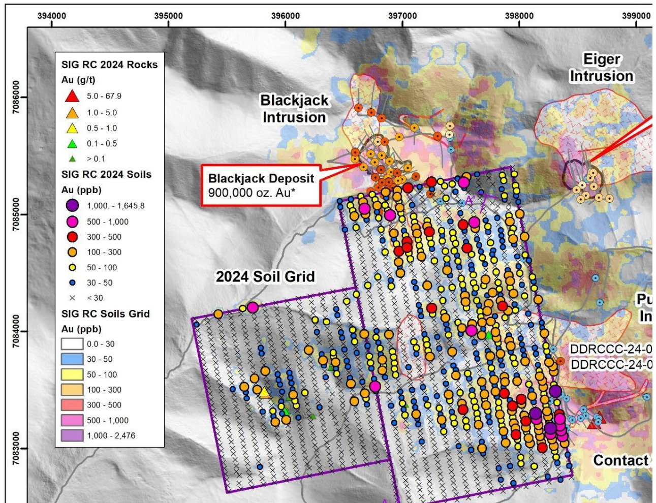
Fig 4 Pukelman Soil Survey & 2024 Drill Hole Location
