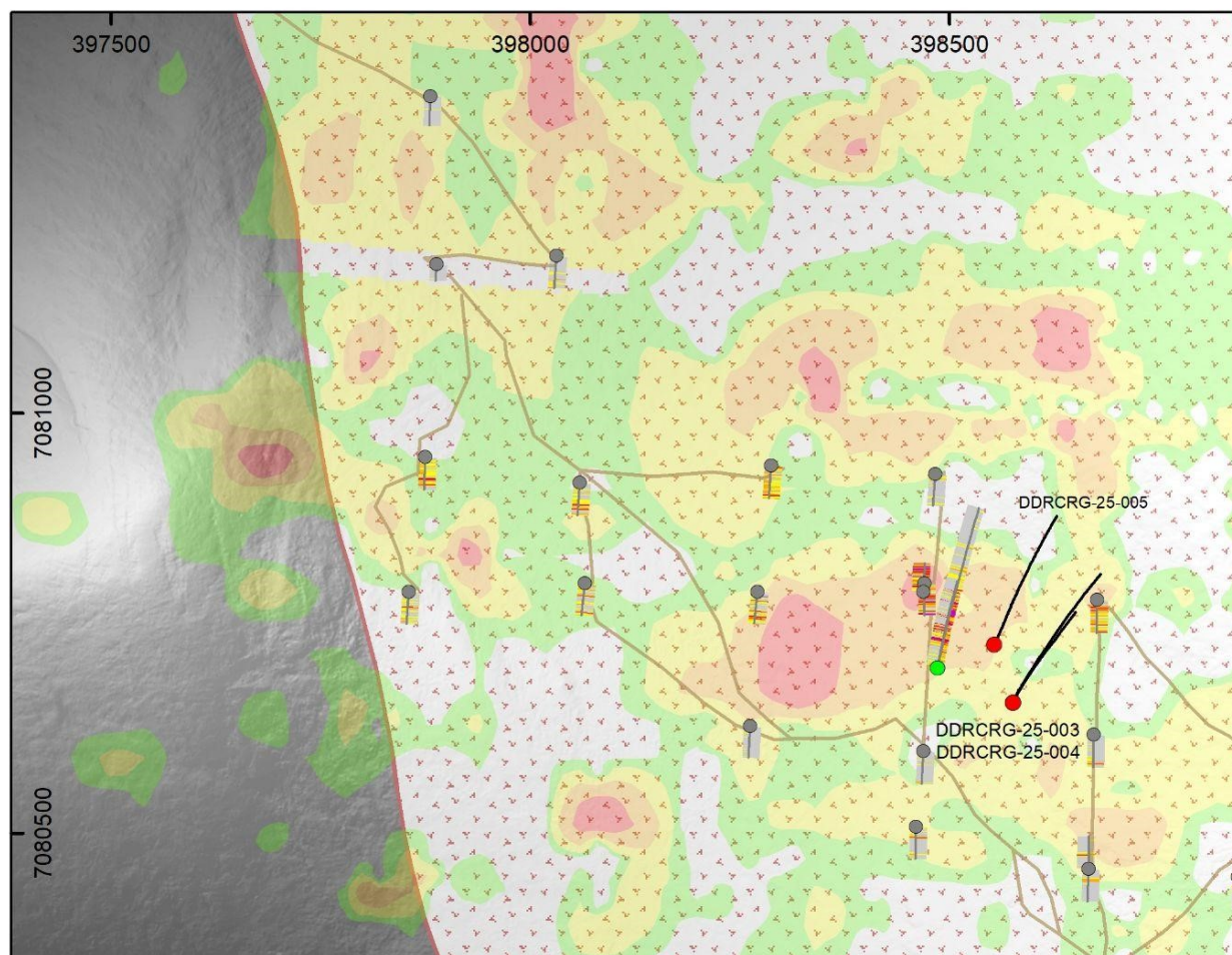
Figure 6: Plan map of the Rhosgobel intrusion showing the 2025 drilling.
