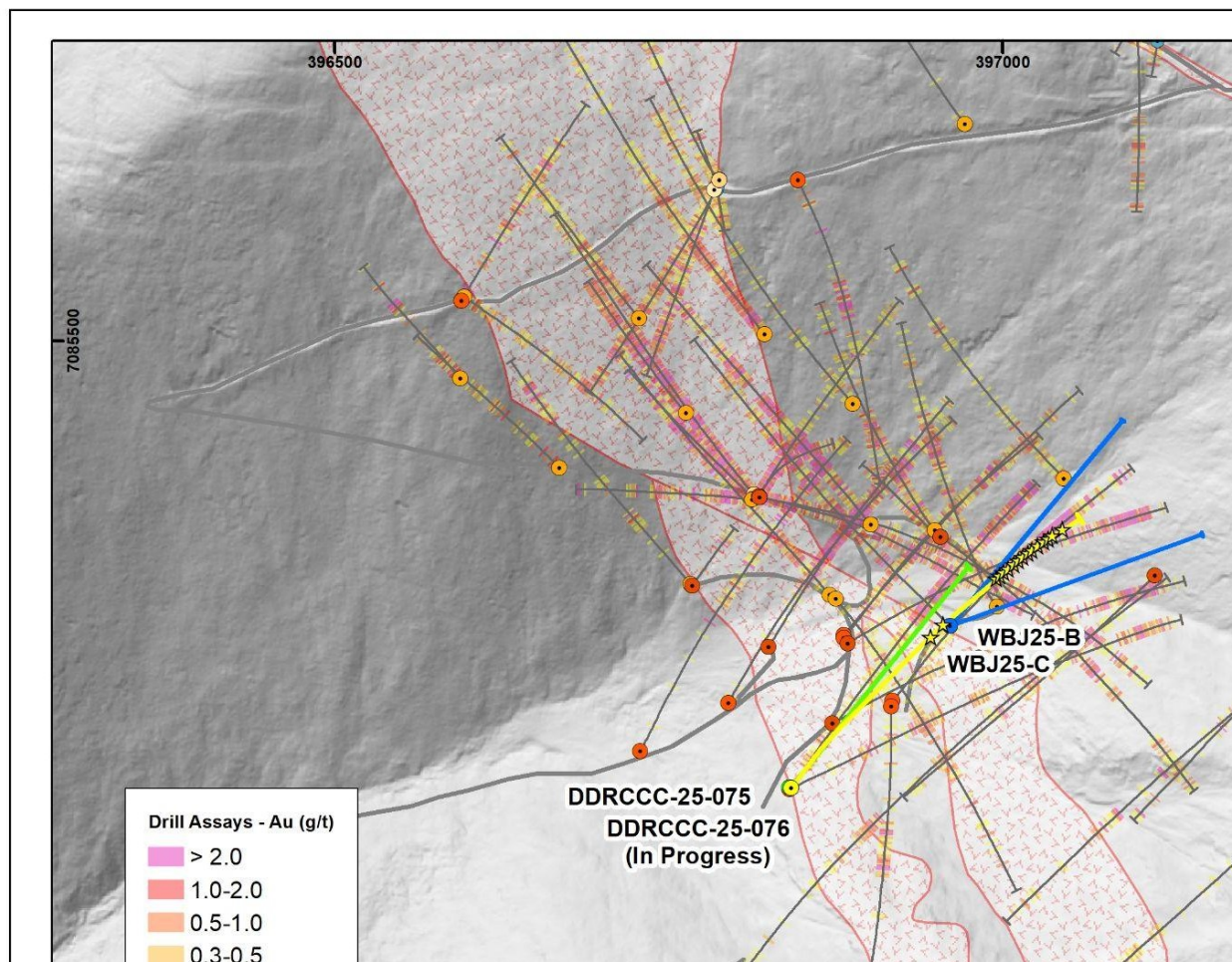
Fig 2A Blackjack Deposit Drill Map 2025
