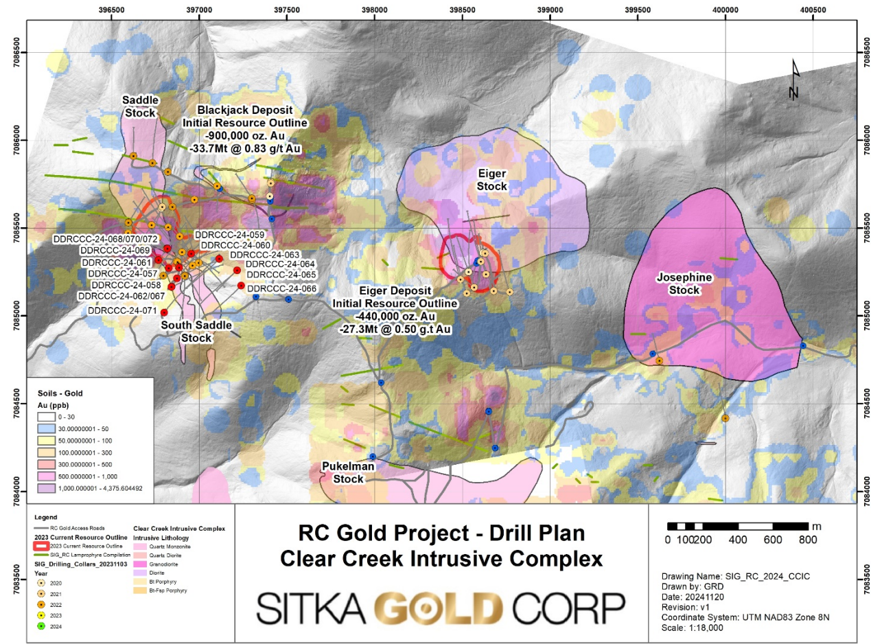
Figure 2: Plan Map of Drill Hole Locations at the Blackjack, Saddle, Eiger and Josephine Zones.
